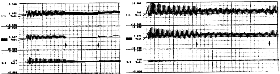
FIGURE 4. (1) Unfiltered P_o , (2) filtered P_o and (3) audio signal during the production of steady state voiced (left) and voiceless (right) trills. The unblocking and blocking of the catheter (area 17.8 \text{ mm}^2 ) is indicated by arrows.
