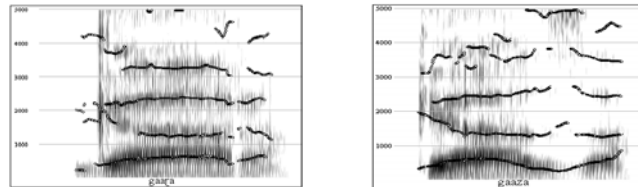
(7) Spectrograms of [ɽ] (left) and [z] (right)
