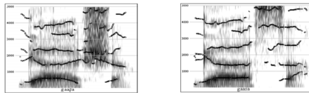
(2) Spectrograms of [ʃ] (left) and [s] (right)
