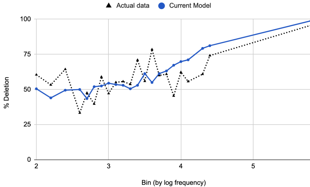
Figure 3. Predicted Percentage Deletion from a model run vs. corpus data
