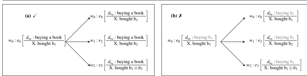
Figure 1 Actual decisions consistent (a) and inconsistent (b) with random choice modal component. (*BOOK w = {b 1 , b 2 , b 1 ⊕ b 2 })
