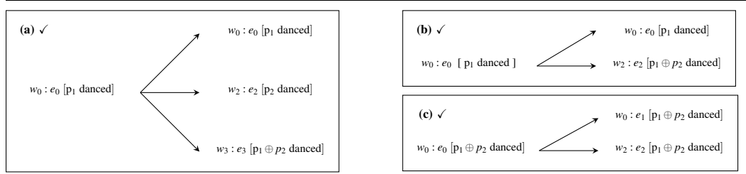
Figure 3 Degrees of ignorance
