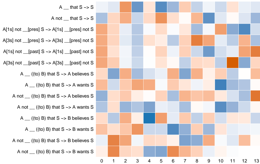
Figure 8 PCA loadings for each inference type.
