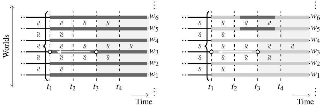
Figure 3 Backshift expansion + forward-extension (Left). The thick dark gray lines indicate that the world-time pairs on these lines are accessible. The domain is further restricted by intersecting with \llbracket \phi \rrbracket and/or propositions obtained through hindsight (Right).
