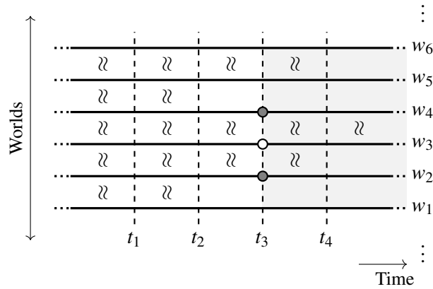
Figure 1 The departing of worlds through time in T \times W -frames.
