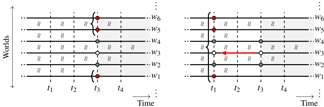
Figure 2 Two ways to expand the quantification domain: vertical expansion (Left, Past-as-Modal) and backshift expansion (Right, Past-as-Past).
